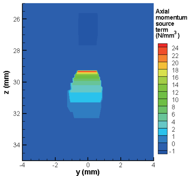
Fig. 3 Axial momentum source term applied to the arc and weld pool to take into account the effect of droplets, in the cross section at x = 0 . The top of the weld pool is at z = 29.3 mm. The welding velocity is to the left.
